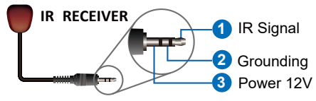
IR RECEIVER
